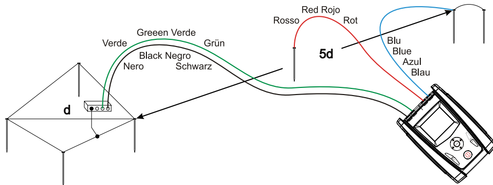
Fig. 6: Earth resistance measurement – small-sized earth rods
