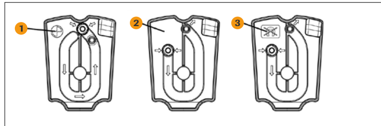
1 Pumped flow plate 2 Non- pumped flow plate 3 PC/Cal test flow plate
