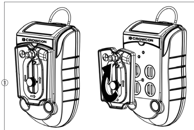
Figure 5: Fitting a flow plate
