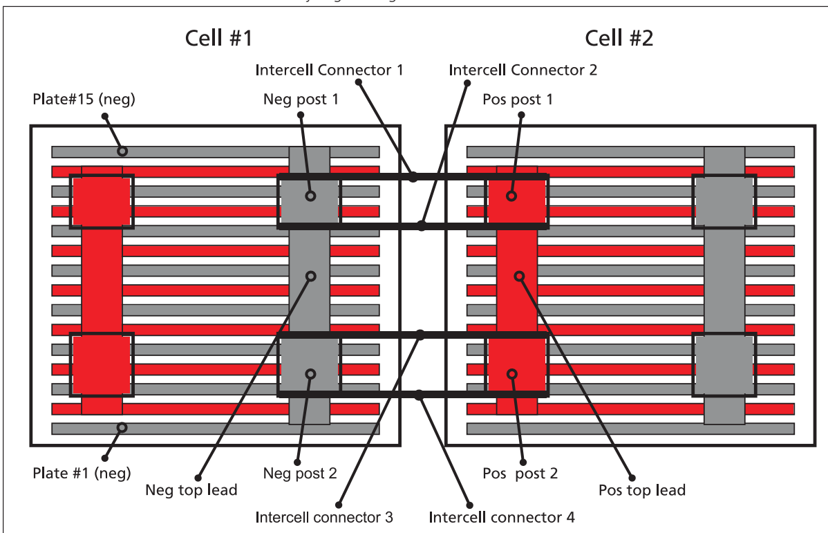
Figure 1 Battery construction diagram
