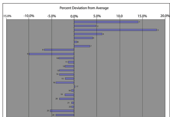
Figure 11 Impedance percent deviation from average
