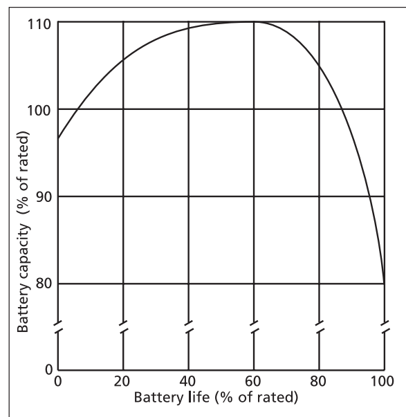
Figure 4 Replacement of battery is recommended when the capacity is 80% of rated.
