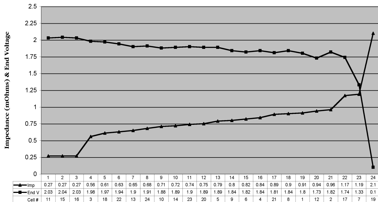
Figure 5 Ascending impedance with corresponding end voltage
