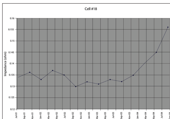
Figure 12 Single cell trending
