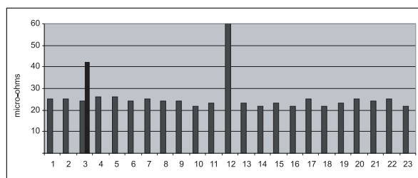
Figure 7 Intercell connection resistance bar graph
