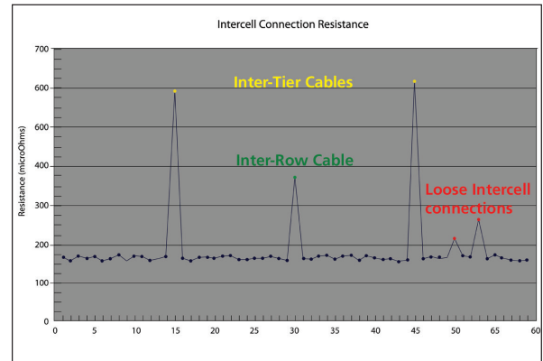
Figure 10 Inter-cell resistance graph
