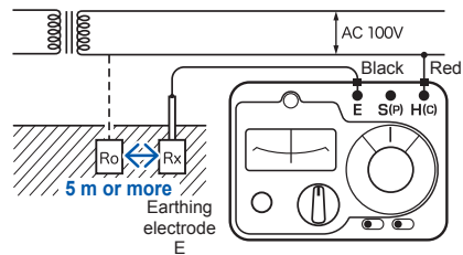
Connection diagram for 2-pole measurement method
