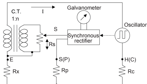
Measurement principle diagram (3-pole measurement)
