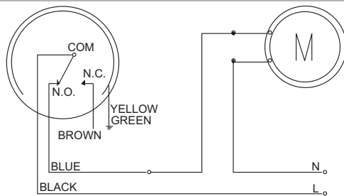
Figure 9-Double Function (Filling (NC)) FSW2-DGXX-XX
