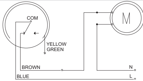
Figure 7-Filling (NC) Function FSW2-CGXX-XX
