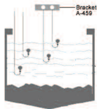
Figure 1: Installation
