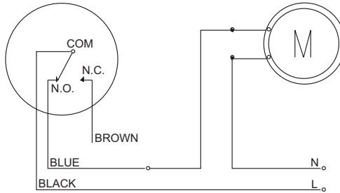
Figure 5-Double Function (Filling (NC)) FSW2-DNXX-XX
