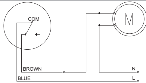
Figure 3-Filling (NC) Function FSW2-CNXX-XX
