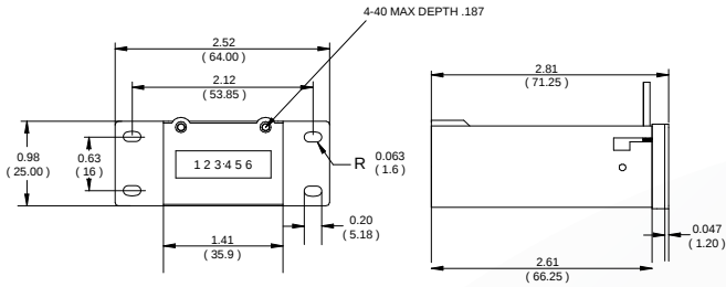
D - D-Base Mount
