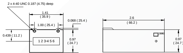
R- Behind The Panel Mount (Front)
