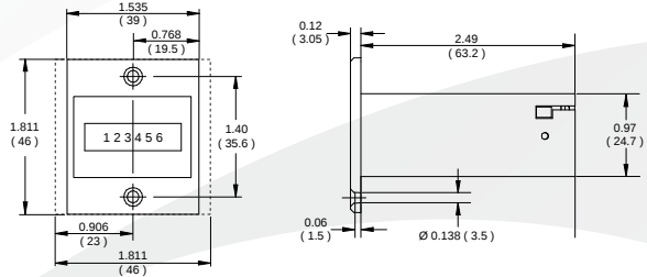
FL - Panel Mount (Flange FL) 1.535 x 1.8 (39 x 45.7) P - Panel Mount (Flange) 1.81 x 1.81(46 x 46)
