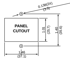
Panel Cutout
