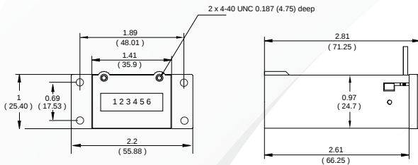
OR - Front / Base Combo Mount (Front)
