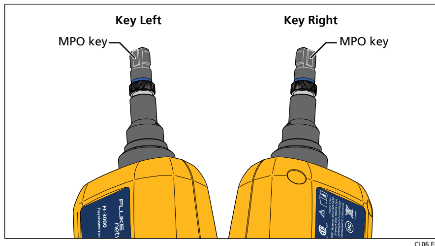
Figure 6. Left and Right Key Positions for the MPO Inspection Tip
