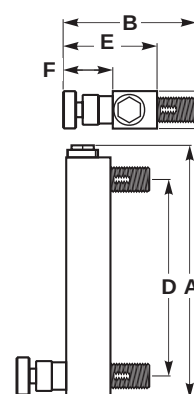
Adjustable Panel Mount
