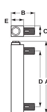
Non-Adjustable Panel Mount
