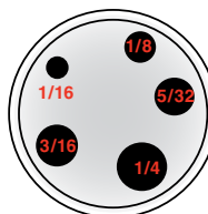
Imperial Multi-hole Type 11 (ETC-400 A)
