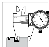
Outside Measurement
