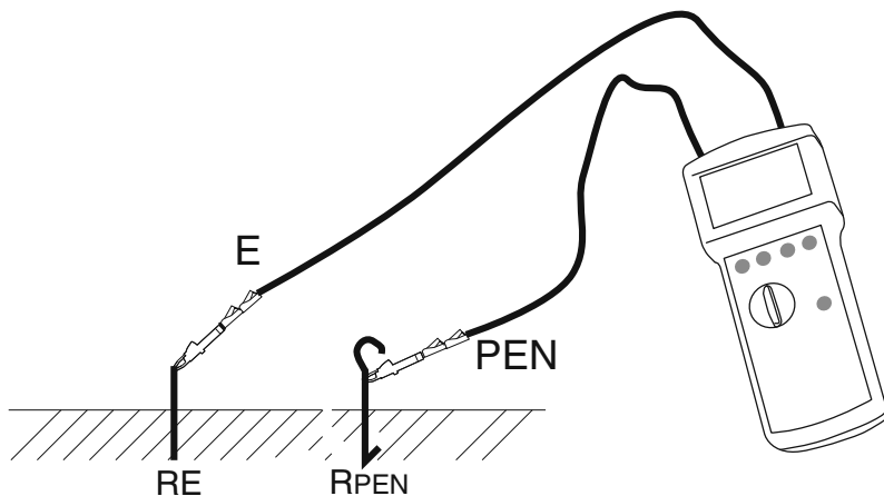
Figure 3: two-wire method
