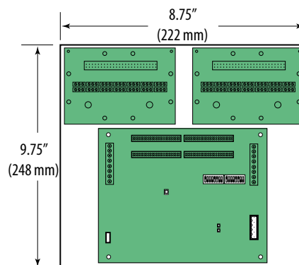
E31xY63 Boards with Bracket
