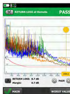
Return loss graph
