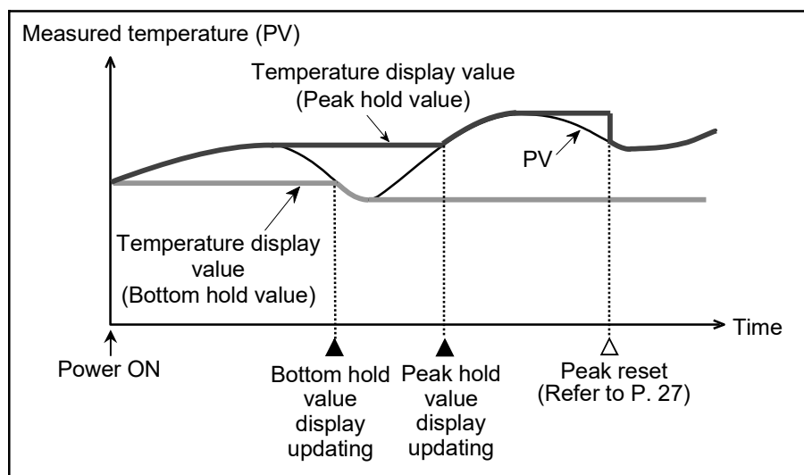
Peak/bottom hold action description
