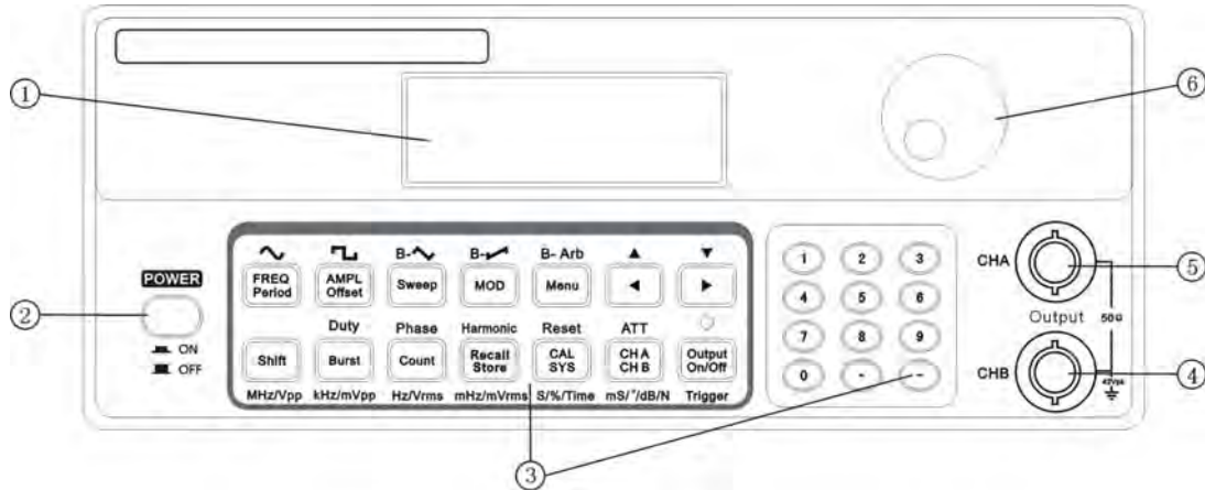
Front panel
