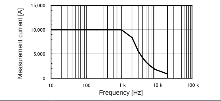
Frequency derating (continuous, design values)
