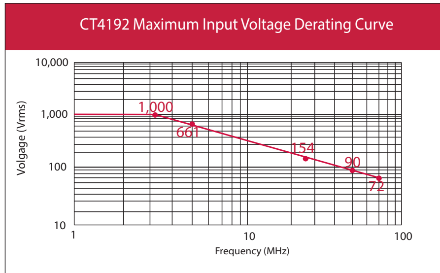
Figure 4 Derating Curve
