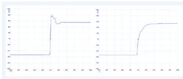
Figure 3: Over/Under Compensation
