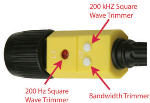
Figure 2: Frequency Compensation Trimmer
