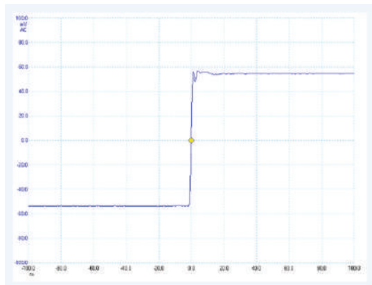
Figure 4: Good Compensation
