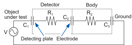
Equivalent circuit diagram
