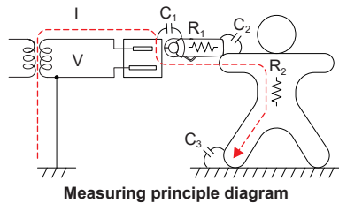
Measuring principle diagram
