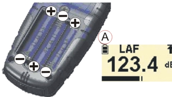
Figure 2: Fitting Batteries
