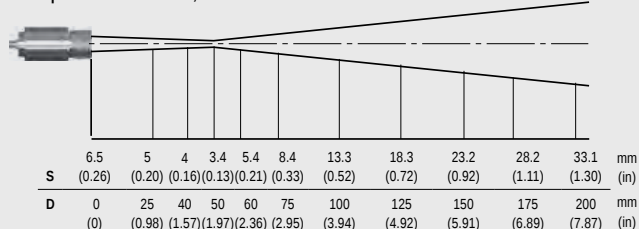
Optics CT LT CF, D:S = 22:1
