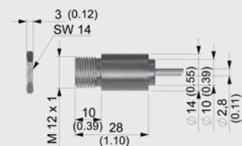
Sensing head (standard)
