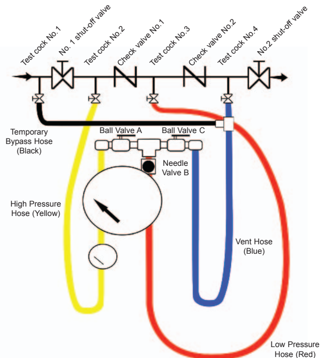
Figure 3 - Reduced Pressure Principle Backflow Preventer
