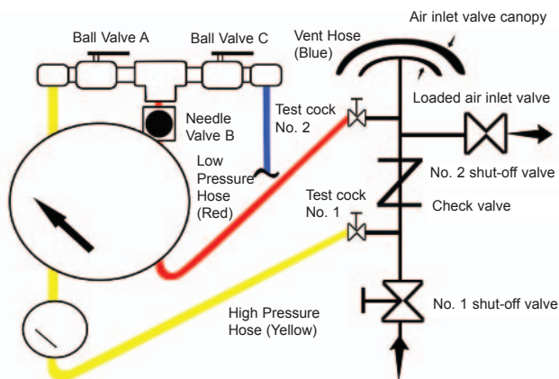
Figure 1 - Pressure Vacuum Breaker
