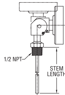
Adjustable Angle Connection
