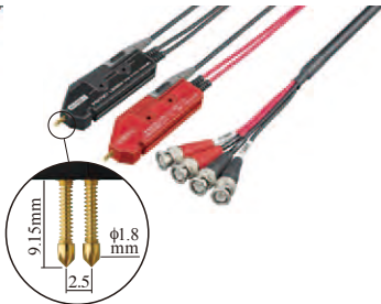
PIN TYPE PROBE L2003 Cable length 1.5 m (4.92 ft)
