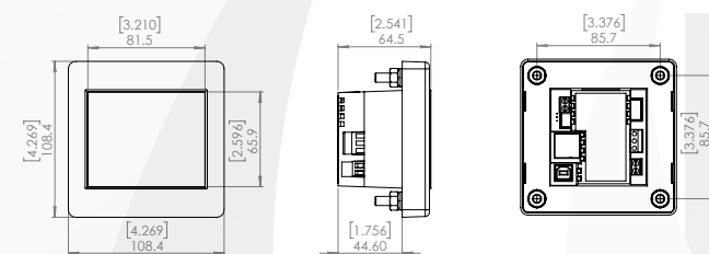
Panel cutout: Square: 68mm x 68mm [2.7" x 2.7"] Circle Diameter: 96mm [3.8"]
