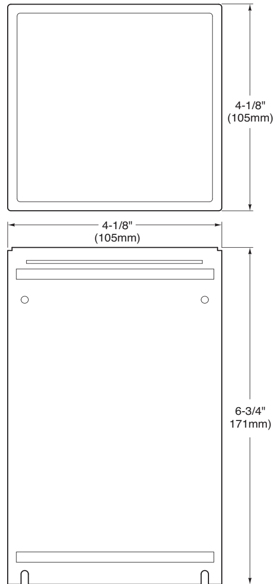
Figure-2 AM-363 Gasket Cover Kit Dimensions.
