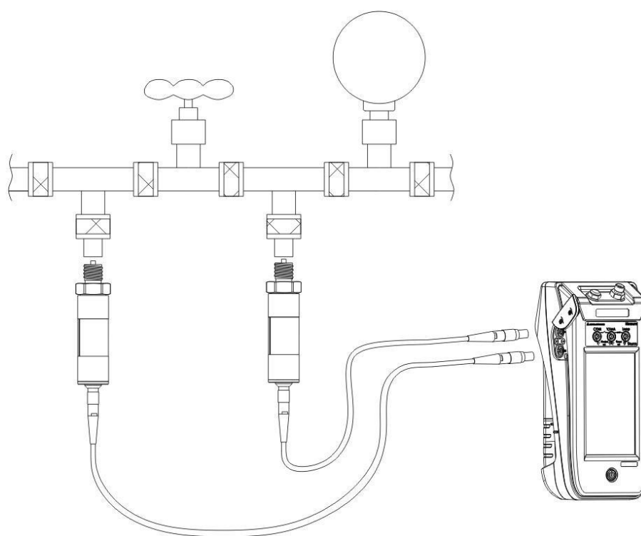
Figure 13 External Pressure Module Connection
