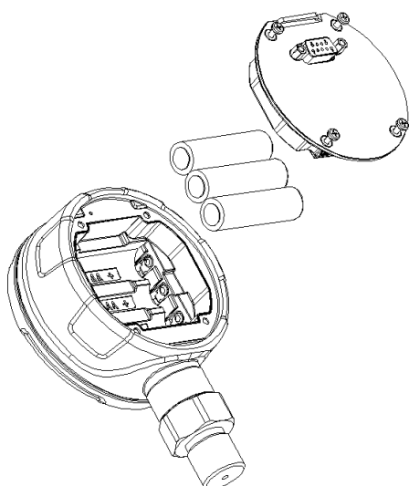
Figure 3 Install batteries
