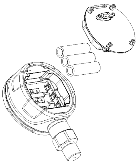
Figure 3 Install batteries
