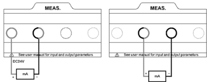
Figure 7 Current Measurement
