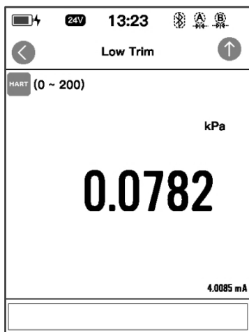
Figure 16 Sensor trim
