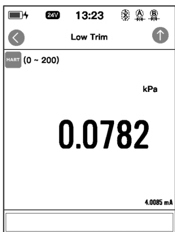
Figure 16 Sensor trim
