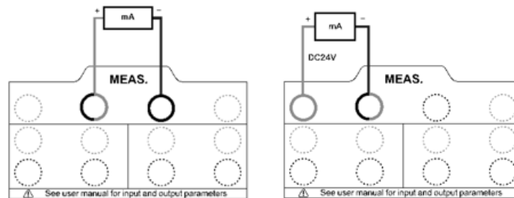
Figure 8 Current measurement
