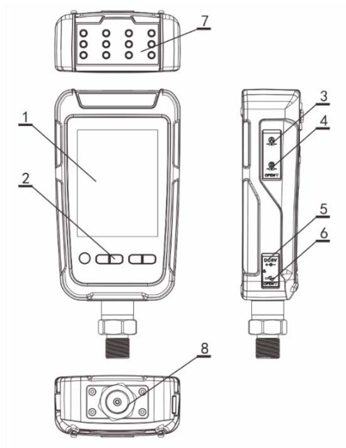
Figure 1 Basic Structure
