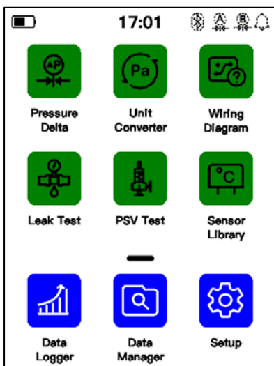
Figure 3 Main interface
