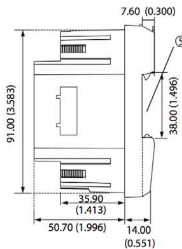
Side View of the DIN rail Meter
