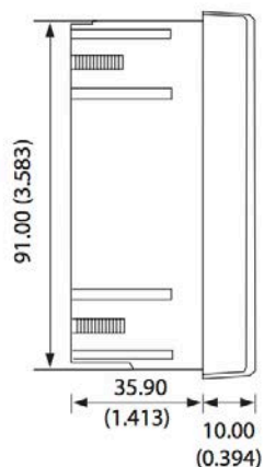
Side View of the Remote Display Unit
