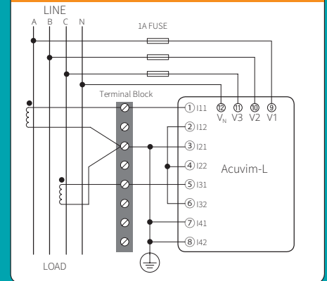
3 Phase 4 Wire (Wiring: 3LN, 3CT; IN: Calculated)
