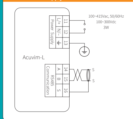
Power Supply + Communication
