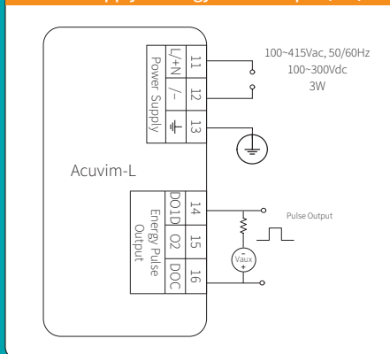
Power Supply + Energy Pulse Output (DO)**
