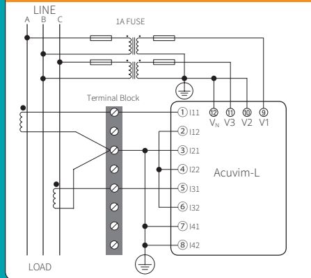
3 Phase 3 Wire (Wiring: 3LL, 3CT)
