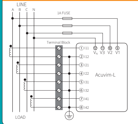
3 Phase 4 Wire (Wiring: 3LN, 3CT; IN: Measured)
