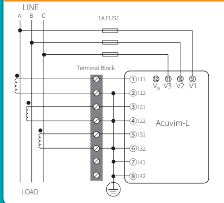
3 Phase 3 Wire (Wiring: 3LL, 3CT)
