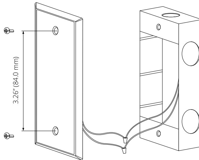
Figure 3 AcuTEMS WP Flying Lead Connection
