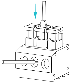
Figure 4 AcuTEMS DM Push Button Terminal Block
