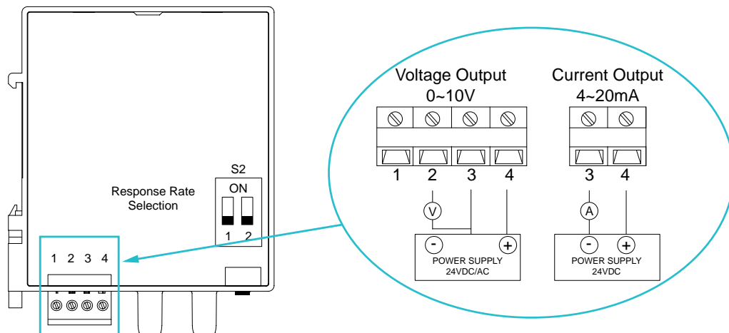
Figure 7 AcuPRE PM Wiring Terminals
