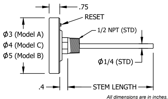
Standard Dimensions
