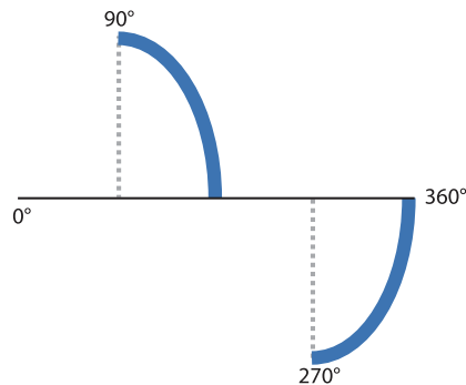
Leading Edge Dimmer at 90°
