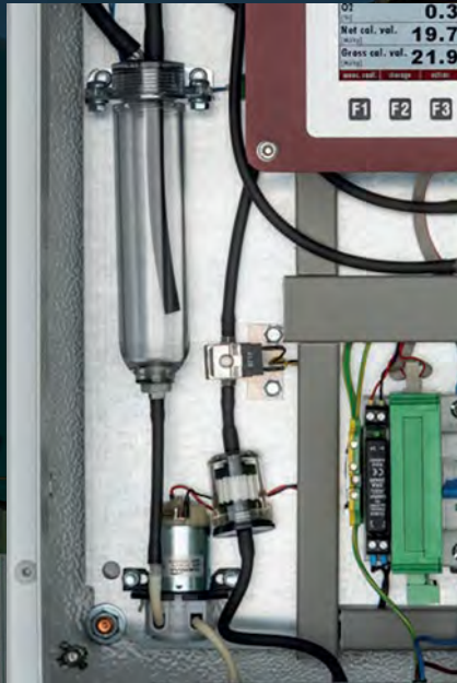
Condensate catch pot and draining pump
