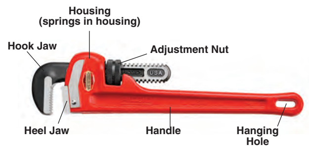
Figure 2 – Wrench Parts
