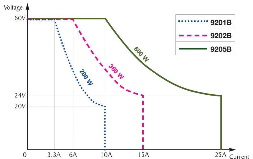
Model 9201B / 9202B / 9205B output characteristics
