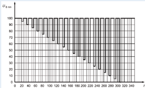
Fig. 3 - Reset behavior voltage drop test
