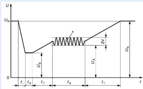
Fig. 4 - Starting profile test
