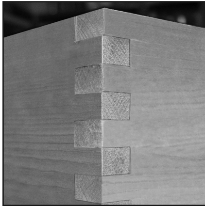
BOX JOINT
