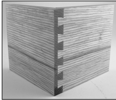
HALF BLIND
