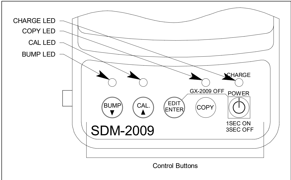
Figure 9: Control Panel
