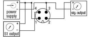
1 switching output (M12x1) with 4 mA to 20 mA signal n-switching
