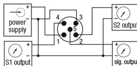
2 switching output (M12x1) with 4 mA to 20 mA signal p-switching
