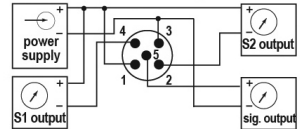
2 switching output (M12x1) with 4 mA to 20 mA signal n-switching
