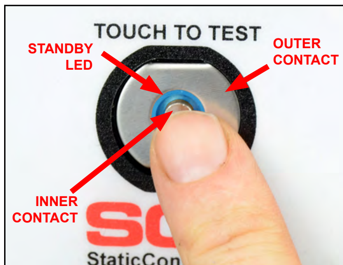
Figure 10. Steady-State Test Switch features and components
