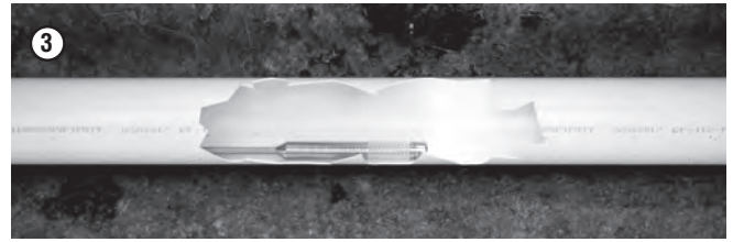
3 RE-INSPECT THE LINE TO ENSURE IT IS FREE OF DEBRIS AND CONFIRM LOCATION AND SIZE OF REPAIR
