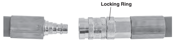
a. Loosen Locking Ring on Female Fitting
